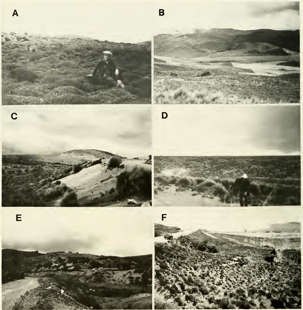
FIG. 10. Habitats of Eleutherodactylus curtipes . Mesic areas on east slope of N. Chimborazo, 3700 m—(A) cushion plants, (B) aspect. Xeric areas, west slope of N. Chimborazo, Arenal, 4150 m—(C-D) dry areas, (E) slightly more moist area. (F) Desierto de Palmira, N of Palmira.
